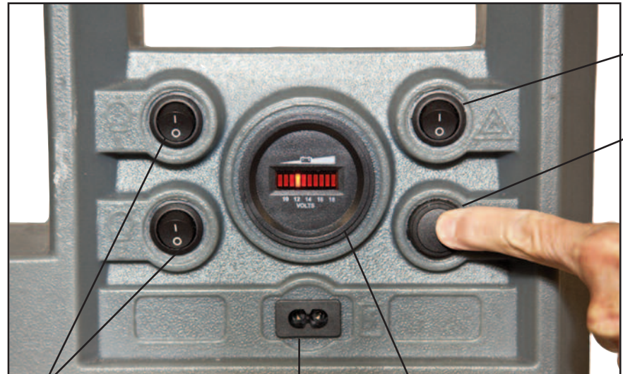
Independent Light On/Off Switches 110 - 240 VAC Charge Jack Voltage Meter
