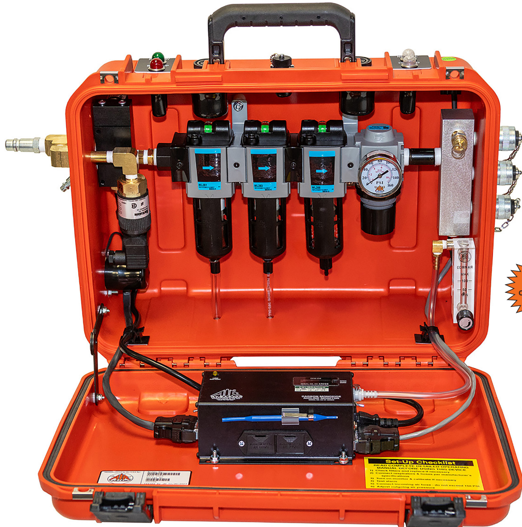
Auto-Air™ Breather Box® Electronic Reserve Air System BB30-COAA
