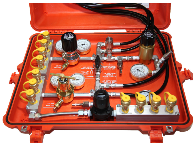
MACK-3™ with optional MACK-3FA fill regulator to fill high pressure cylinders
